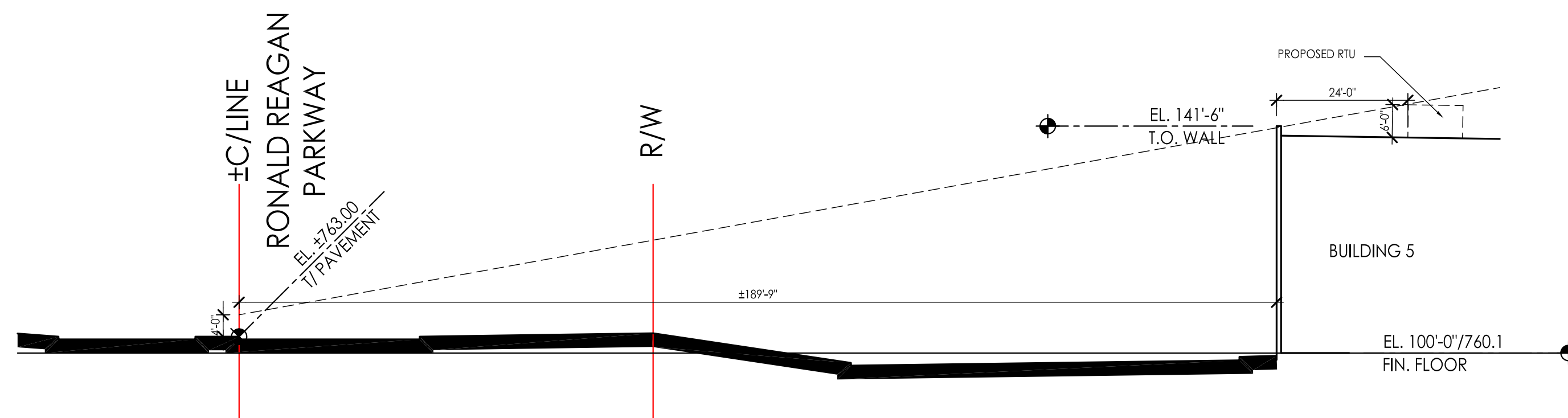
CROSS SECTION GG
