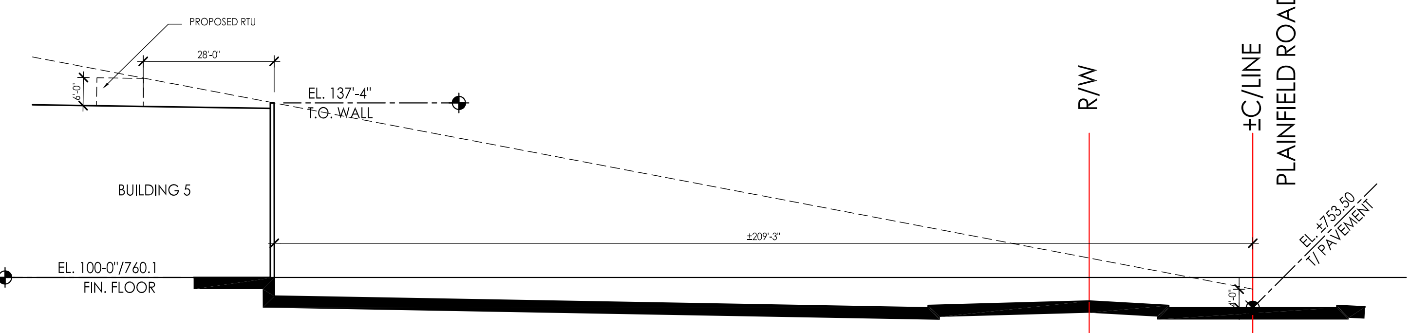
CROSS SECTION HH
