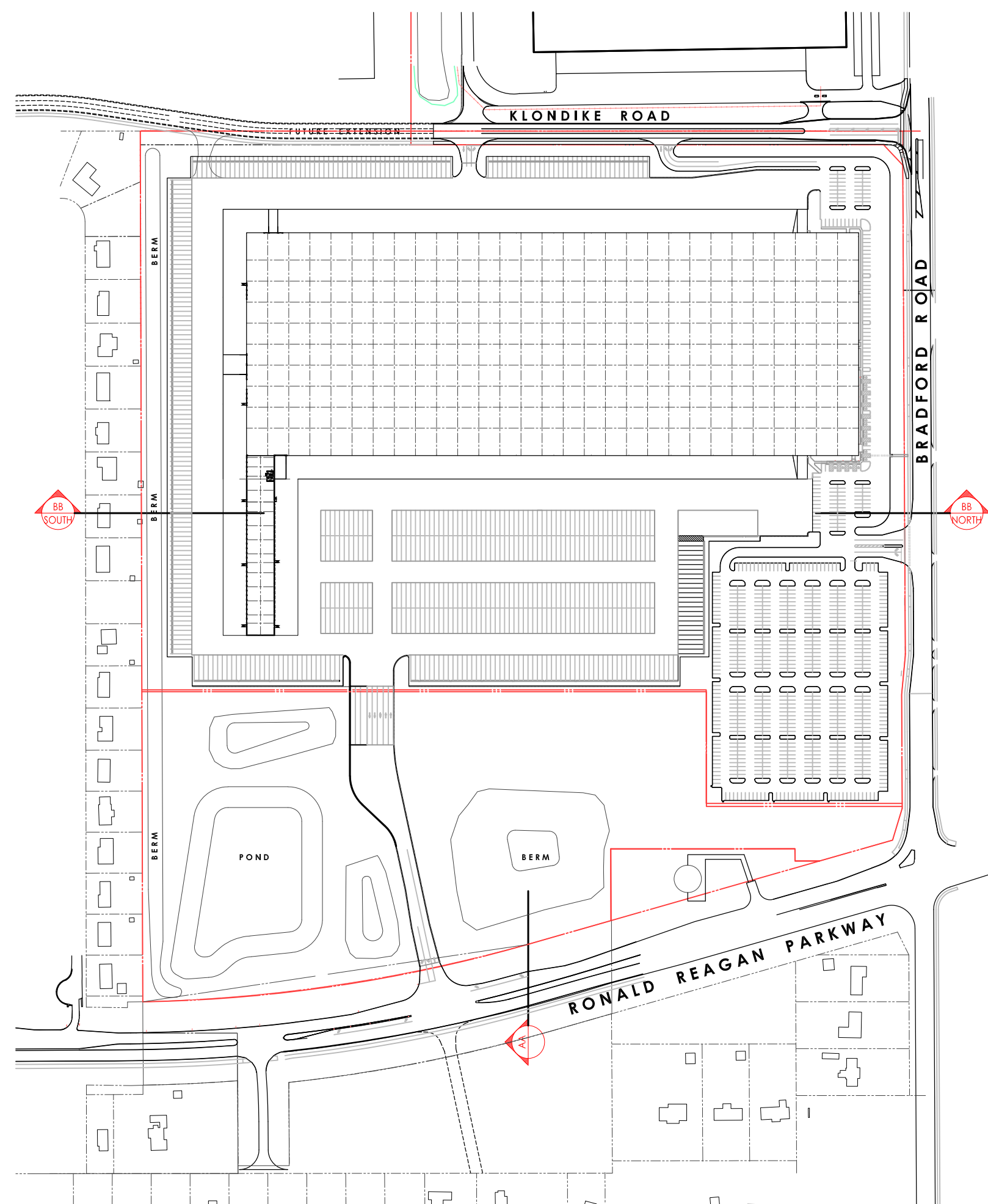
LOCATION PLAN
