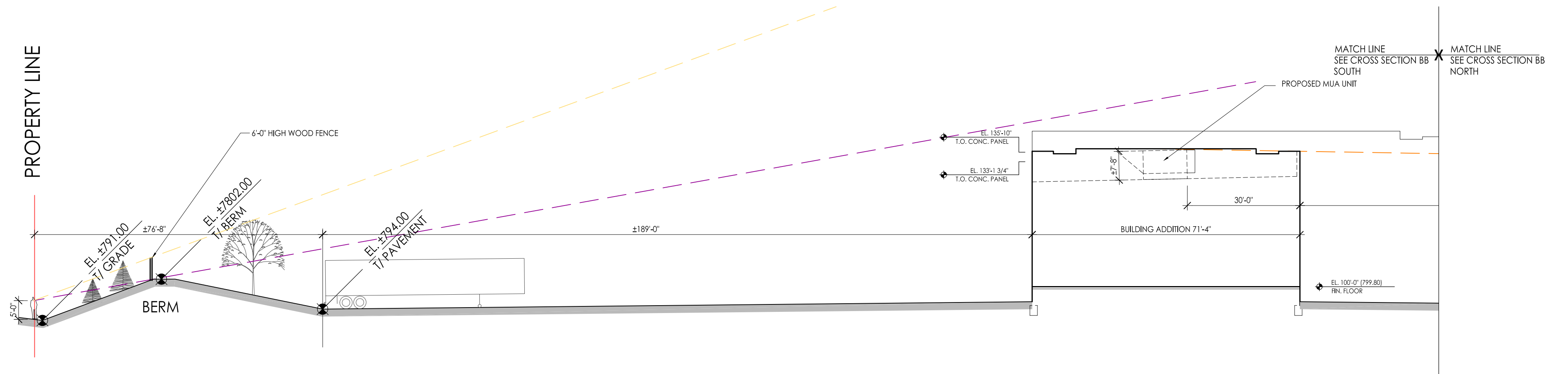
CROSS SECTION BB - SOUTH
