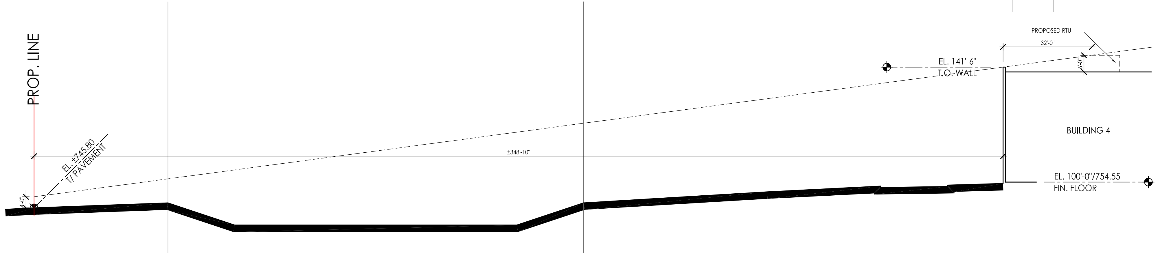
CROSS SECTION AA 1" = 20'-0" 0 5 10 20 40'
